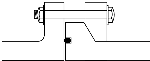
Figure 4-12 Loose ring flange with O-ring gasket
