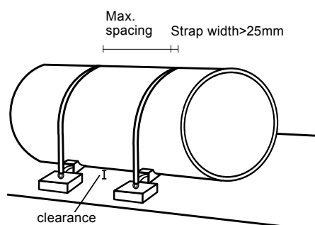
Figure 5–2 Pipe anchoring – Maximum spacing of straps see table Table 5–2
