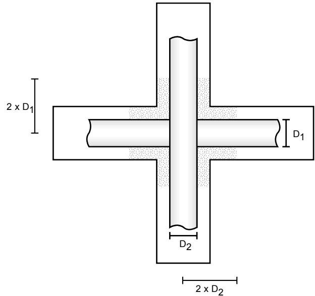
Figure 7-3 Top view of backfill in cross-over.
