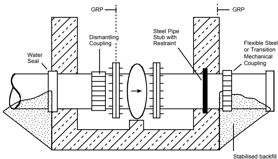
Figure 8–5 Anchoring
