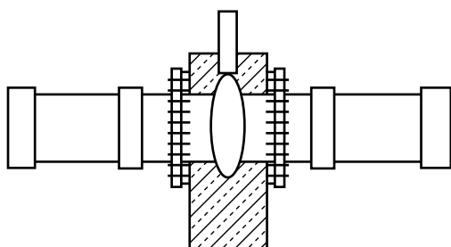
Figure 8-1 Type I – Valve encased in thrust block
