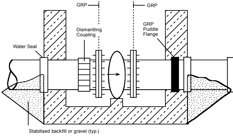
Figure 8-4 Type IV – Use of puddle flange to accommodate thrust forces
