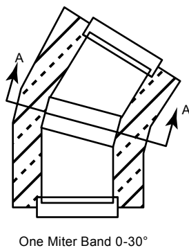
Figure 5-1 Thrust blocks
