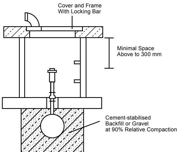
Figure 8–6 Accommodating a small diameter air/vacuum valve
