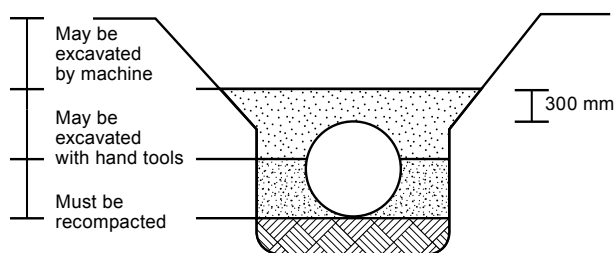
Figure 9-2 Excavating over-deflected pipe
