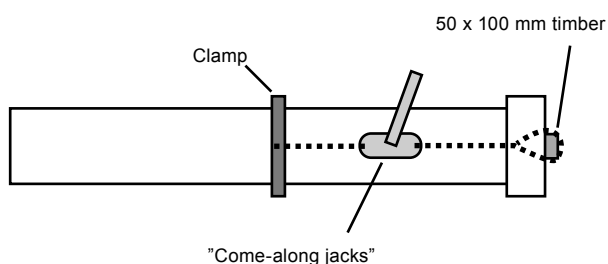
Figure 4-5 Mounting of coupling on pipe
