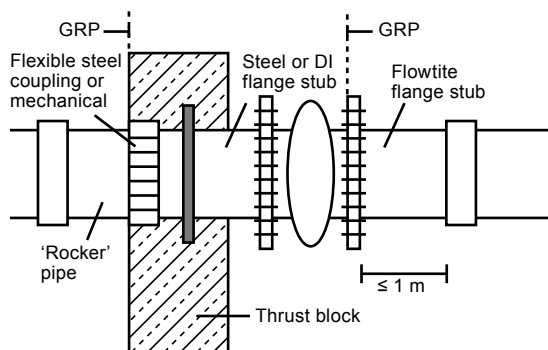
Figure 8-2 Type II – Thrust block adjacent to valve
