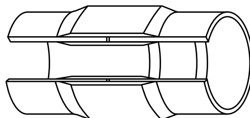
Figure 4-14 Lay-up joint
