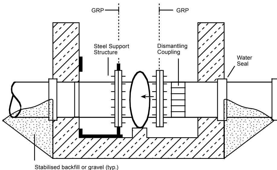
Figure 8-3 Type III – Use of structural support system to accommodate thrust forces
