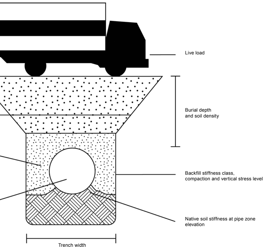
Figure A-1 Installation Design Parameters
