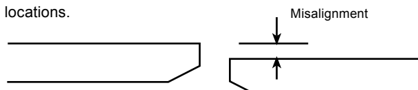
Figure 4-9 Misalignment
