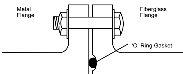
Figure 4-11 Flanged joint
